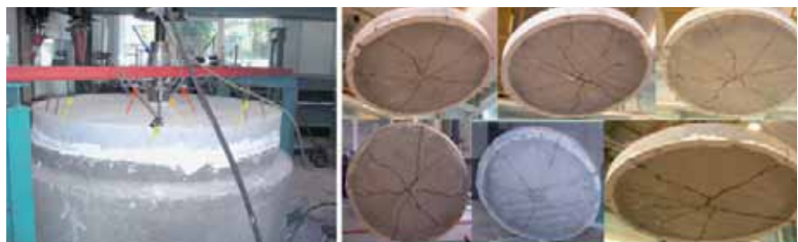
Figure 6: Round slab test set-up (left) and typical fan pattern cracking (right).
