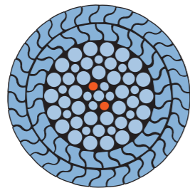
FLC track ropes with optical fibres for data transmission
