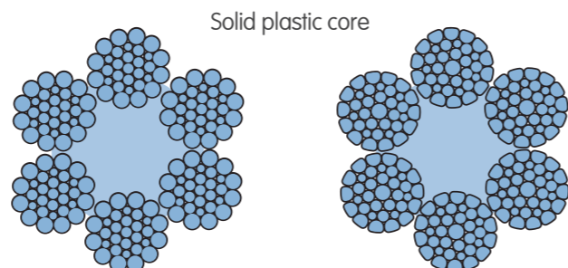
6x31 WS
