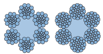
6x26 WS
