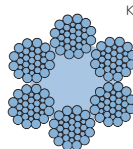
6x31 WS
