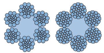
6x26 WS
