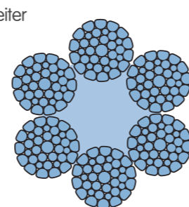
6x36 WSR
