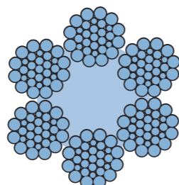
6x31 WS
