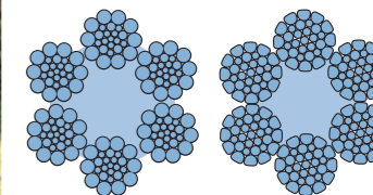
6x26 WS
