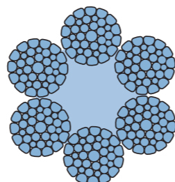
6x36 WSR
